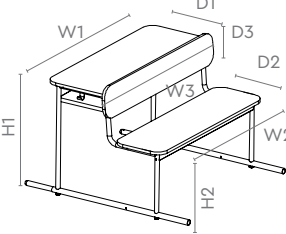
Genii Compact Laminate Middle Module
