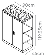
KD Minor (with Laminate Top)
