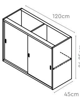
VSDU-10 (with Metal Top)
