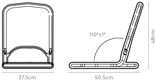
Open Seat Back Condition
