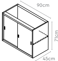
VSDU-6 (with Metal Top)
