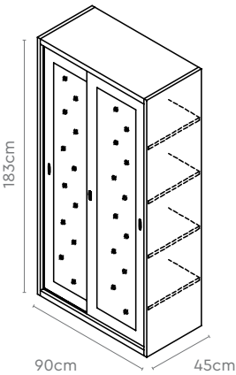
VSDU-8 (with Metal Top)
