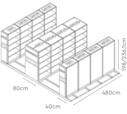
M4 Motorized with Platform
