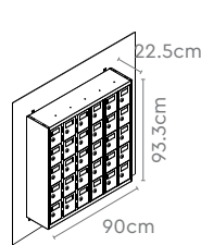
30 Door Locker Wall Mounted
