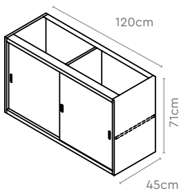
VSDU-12 (with Metal Top)
